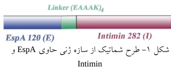
Figure 1. Schematic diagram of gene construct containing EspA and Intimin
